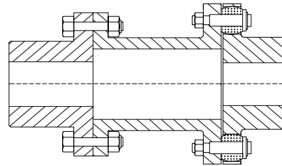
Spacer Coupling
